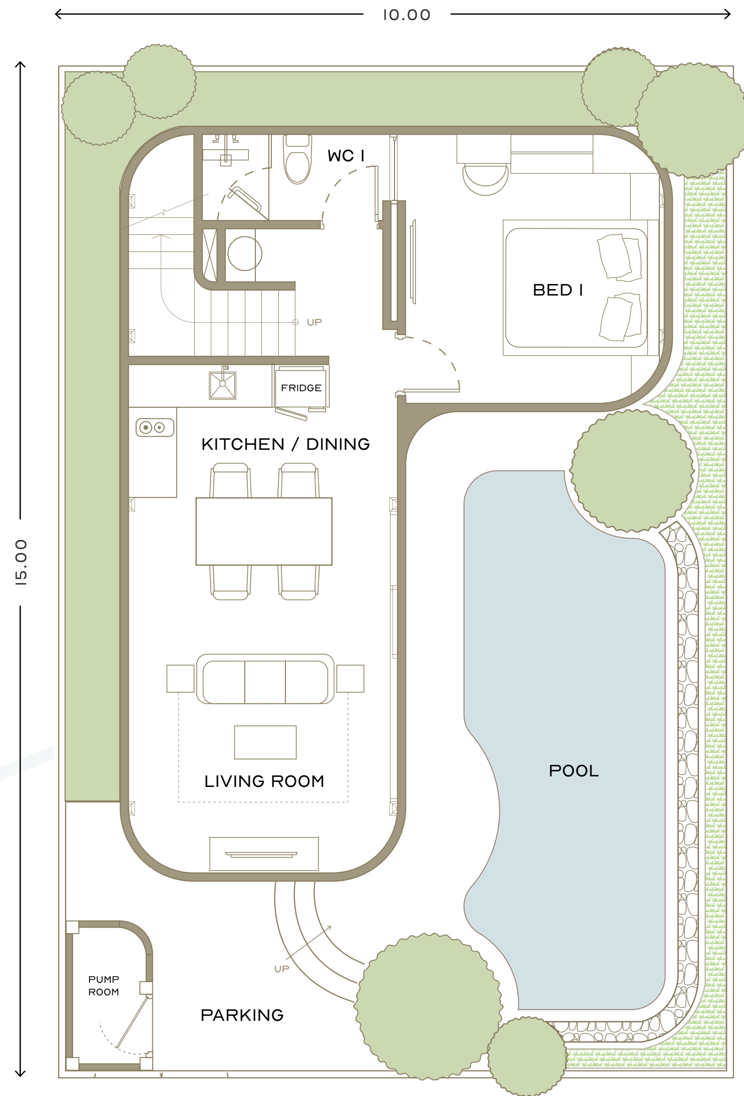
GROUND FLOOR
